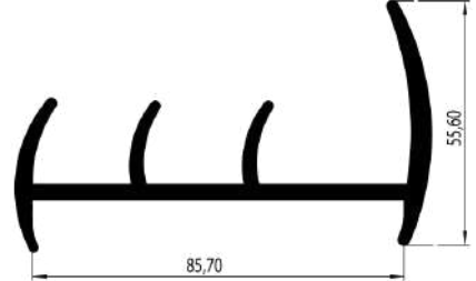
Lp 85 Lp Profile
