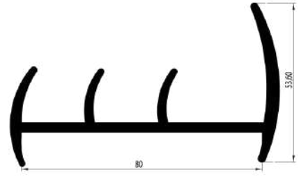
Lp 80 Oluklu Lp Profile
