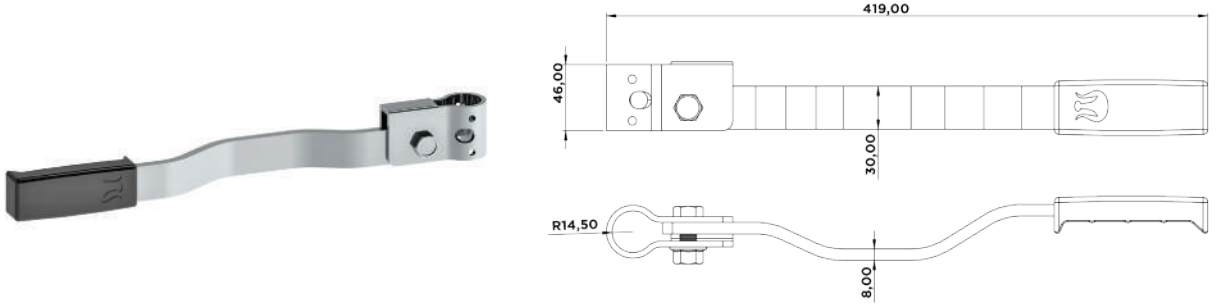
Lama Kol Topuzlu 27 mm Flat Lever With Mounth 27 mm
