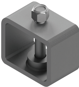
Römork Makas Aparatı Pernolu Spring Fixture With Pin
