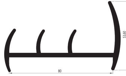
Lp 80 Oluklu Lp Profile
